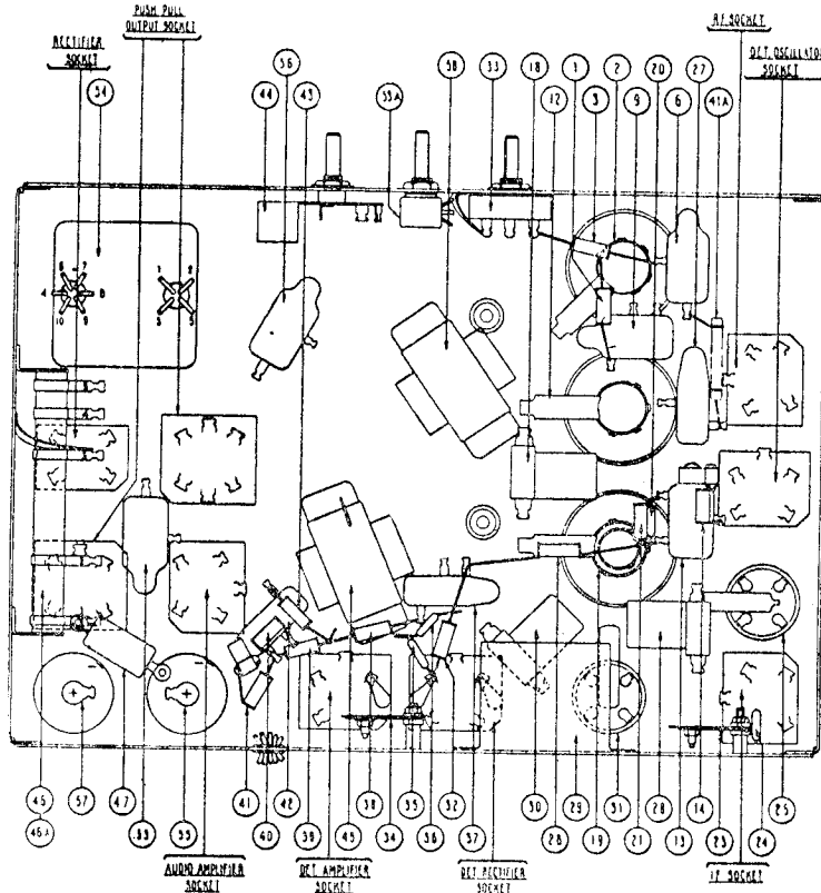
Fig. 5—Parts Diagram
